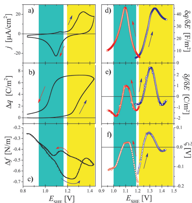
Figure 2. Results for oxygen electroadsorption on Au in 10 mM \text{H}_2\text{SO}_4 at 5 \text{ mV s}^{-1} . a) Cyclic voltammogram. b) Change in charge density \Delta q versus E . c) Change in surface stress \Delta f versus E . d) and e) graphs of the experimental derivatives \delta q/\delta E and \delta f/\delta E versus E . f) The coupling coefficient \zeta versus E , computed from the derivatives according to Equation (2). Arrows indicate sweep direction; color shades highlight oxygen adsorption (yellow) and desorption (cyan) processes.
