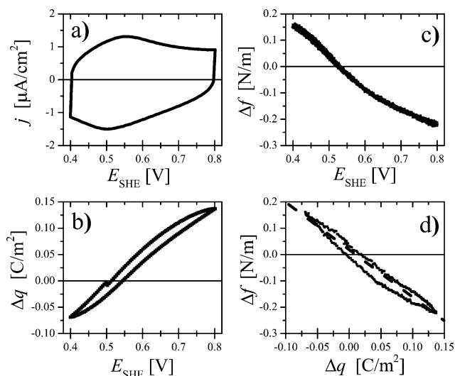
Figure 1. Results for Au in 10 mM \text{H}_2\text{SO}_4 at 5 \text{ mV s}^{-1} within the double-layer regime. a) Cyclic voltammogram of current density j versus potential E . b) Charge density \Delta q versus E . c) Change in surface stress \Delta f versus E . d) Graph of \Delta f versus \Delta q . Dashed line: best fit; slope indicates \zeta = -1.81 \pm 0.02 \text{ V} .
